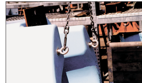
Step 9: Once concrete filled basin is resting in a vertical position, switch lifting rigging from single hoist plate* / fastout device** to double lifting eyes. Do NOT lift basin! Slowly lower basin to rest upright on level ground***
